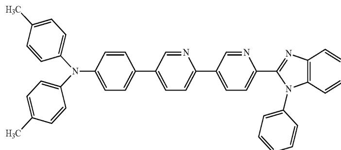
4-methyl-N-(4-(6'-(1-phenyl-1H-benzo[d]imidazol-2-yl)-[2,3'-bipyridin]-5-yl)phenyl)-N-(p-tolyl)aniline,
