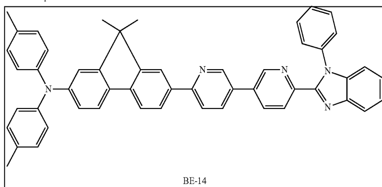
Compound 35
