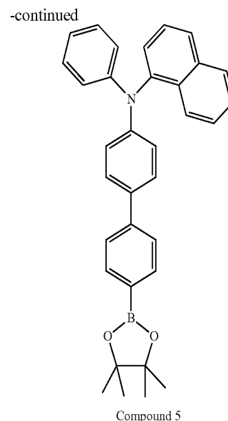
N-phenyl-N-(4'-(4,4,5,5-tetramethyl-1,3,2-dioxaborolan-2-yl)-[1,1'-biphenyl]-4-yl)naphthalen-1-amine (Compound 5)
