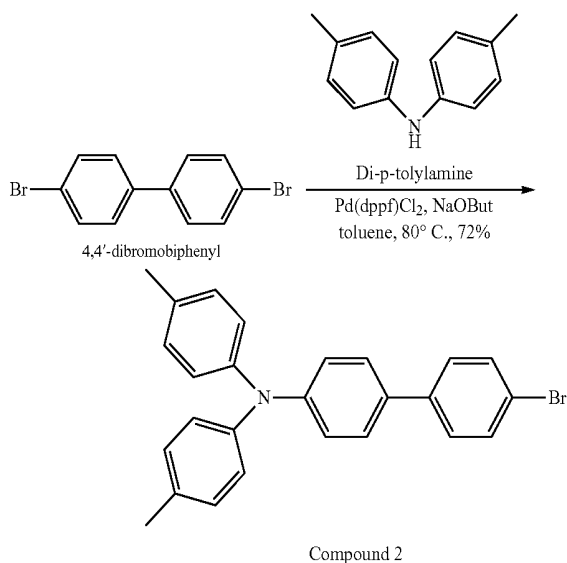
4'-bromo-N,N-di-p-tolylbiphenyl-4-amine (Compound 2)
