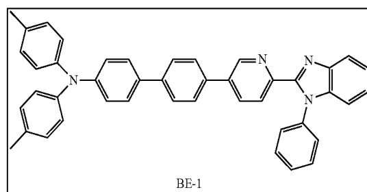
Chemical Formula: \text{C}_{44}\text{H}_{34}\text{N}_4 Molecular Weight: 618.77
