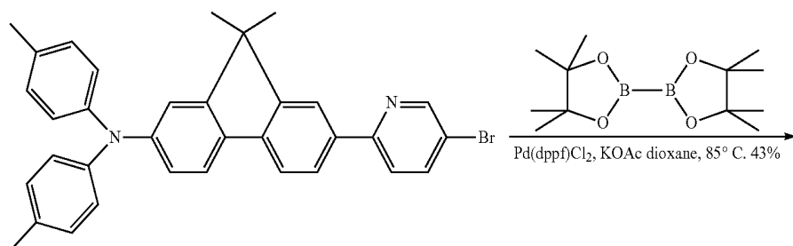
Compound 34
