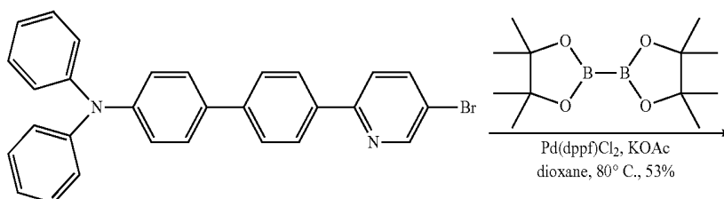
Compound 14
