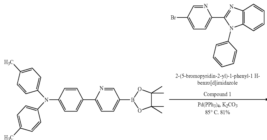
Compound 28
