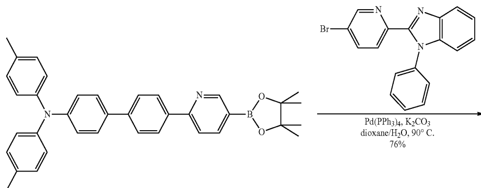
Compound 7
