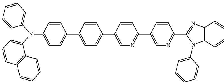
N-phenyl-N-(4'-(6'-(1-phenyl-1H-benzo[d]imidazol-2-yl)-[2,3'-bipyridin]-5-yl)-[1,1'-biphenyl]-4-yl)naphthalen-1-amine,
