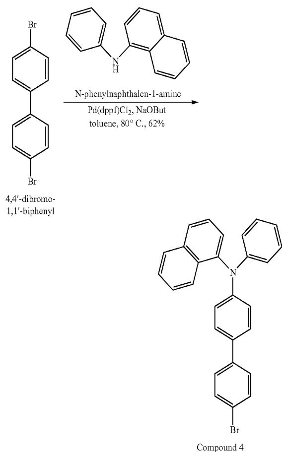
N-(4'-bromo-[1,1'-biphenyl]-4-yl)-N-phenylnaphthalen-1-amine (Compound 4)
