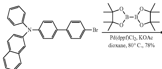
Compound 21
