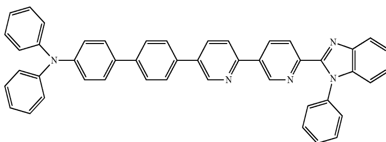
N,N-diphenyl-4'-(6'-(1-phenyl-1H-benzo[d]imidazol-2-yl)-[2,3'-bipyridin]-5-yl)-[1,1'-biphenyl]-4-amine,
