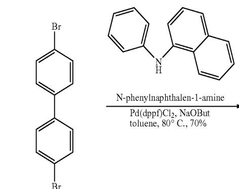
4,4'-dibromo-1,1'-biphenyl
