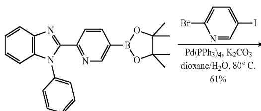
Molecular Weight: 397.28 Compound 10
