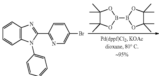
Compound 1
