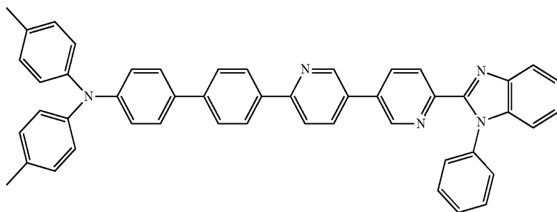
4'-(6'-(1-phenyl-1H-benzo[d]imidazol-2-yl)-[3,3'-bipyridin]-6-yl)-N,N-di-p-tolyl-[1,1'-biphenyl]-4-amine,
