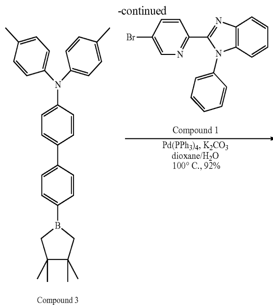
Compound 3
