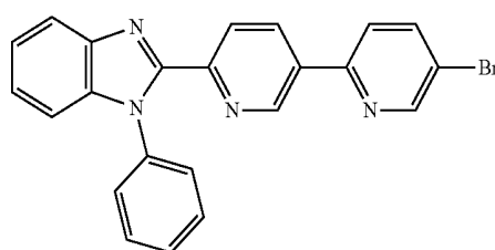
Compound 17
