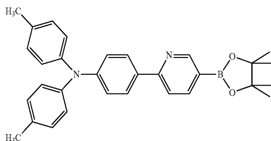
Compound 28
