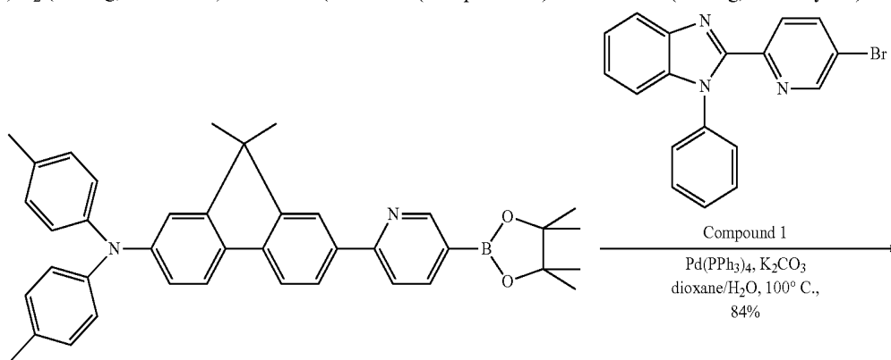
Compound 35
