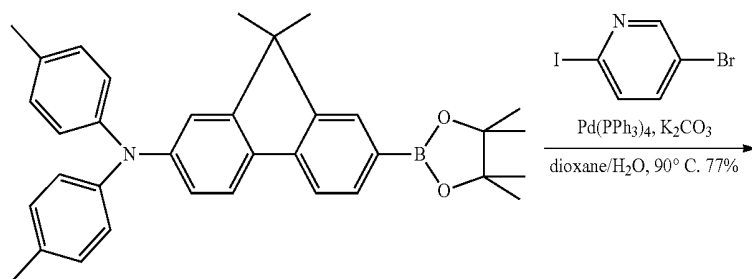
Compound 33
