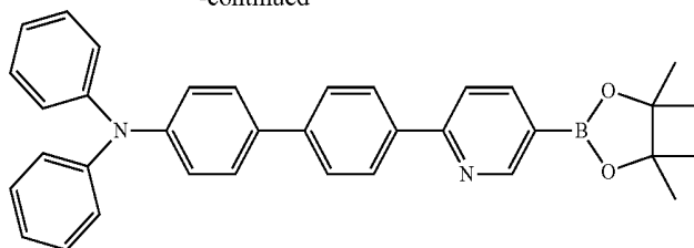
Compound 15
