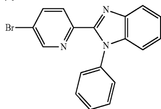
Compound 1
