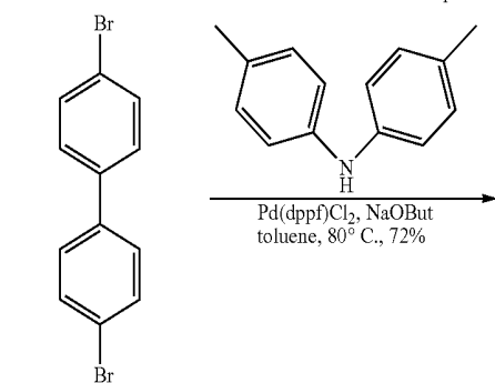
Compound 1
