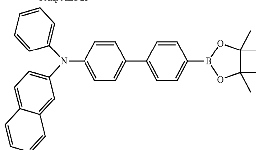
Compound 22
