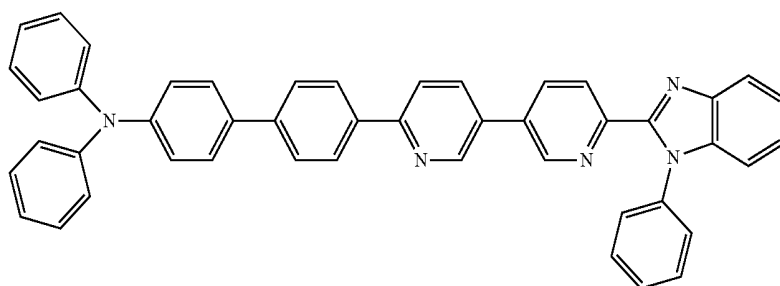
N,N-diphenyl-4'-(6'-(1-phenyl-1H-benzo[d]imidazol-2-yl)-[3,3'-bipyridin]-6-yl)-[1,1'-biphenyl]-4-amine,
