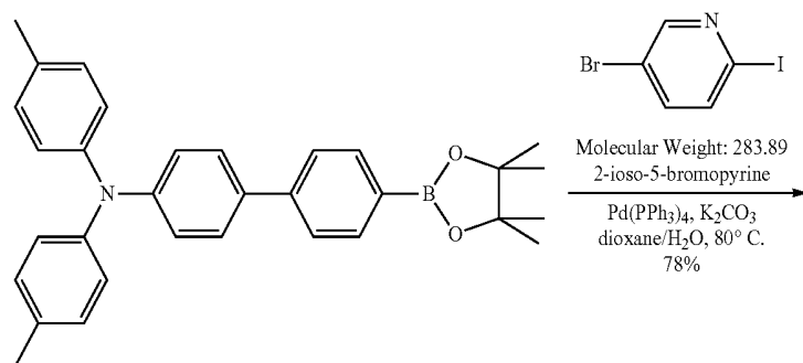
Compound 3
