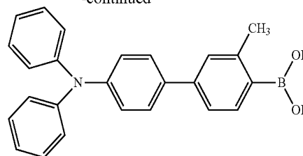
Compound 19 Molecular Weight: 414.34
