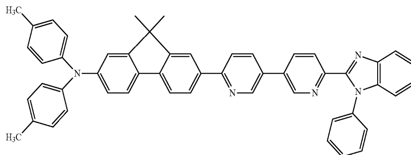
9,9-dimethyl-7-(6'-(1-phenyl-1H-benzo[d]imidazol-2-yl)-[3,3'-bipyridin]-6-yl)-N,N-di-p-tolyl-9H-fluoren-2-amine
