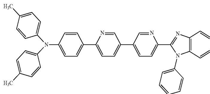
4-methyl-N-(4-(6'-(1-phenyl-1H-benzo[d]imidazol-2-yl)-[3,3'-bipyridin]-6-yl)phenyl)-N-(p-tolyl)aniline,
