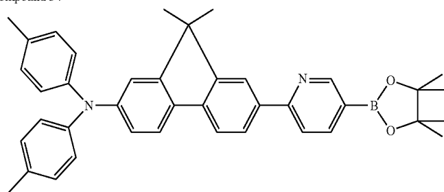
Compound 35
