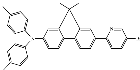
Compound 34
