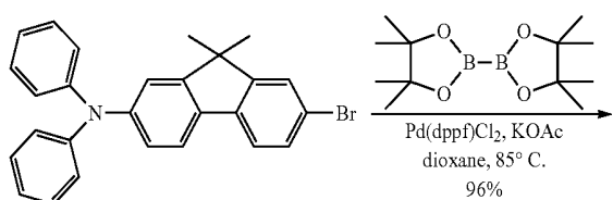
Molecular Weight: 440.37 Compound 8
