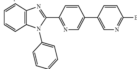
Molecular Weight: 397.28 Compound 10
