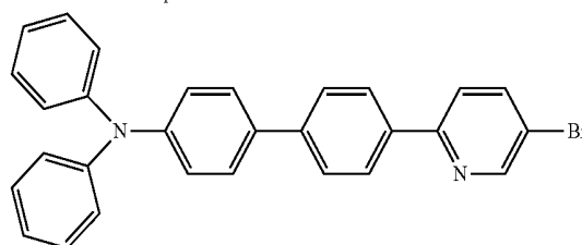
Compound 14
