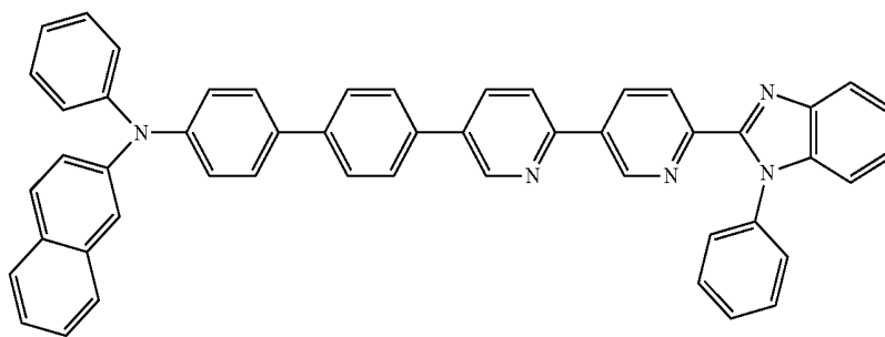
N-phenyl-N-(4'-(6'-(1-phenyl-1H-benzo[d]imidazol-2-yl)-[2,3'-bipyridin]-5-yl)-[1,1'-biphenyl]-4-yl)naphthalen-2-amine,
