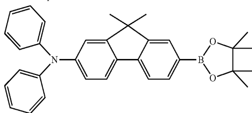
Compound 9
