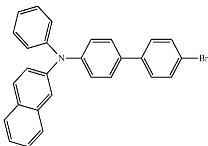
Compound 21 N-(4'-bromo-[1,1'-biphenyl]-4-yl)- N-phenyl-N-(1-phenyl-2-naphthyl)amine
