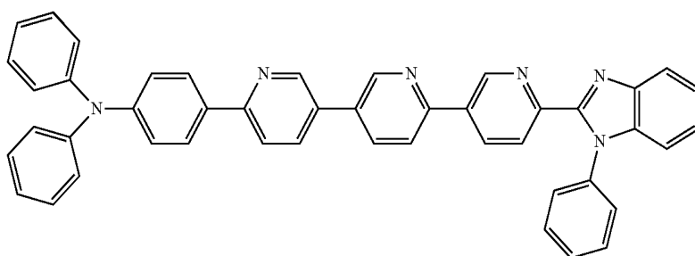
N,N-diphenyl-4-(6-(1-phenyl-1H-benzo[d]imidazol-2-yl)-[3,2':5',3''-terpyridin]-6''-yl)aniline,
