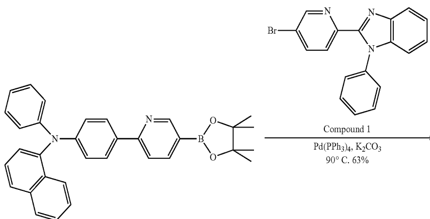
Compound 31
