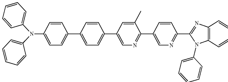
4'-(3-methyl-6'-(1-phenyl-1H-benzo[d]imidazol-2-yl)-[2,3'-bipyridin]-5-yl)-N,N-diphenyl-[1,1'-biphenyl]-4-amine,
