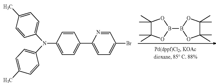
Compound 27
