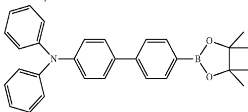
Compound 13
