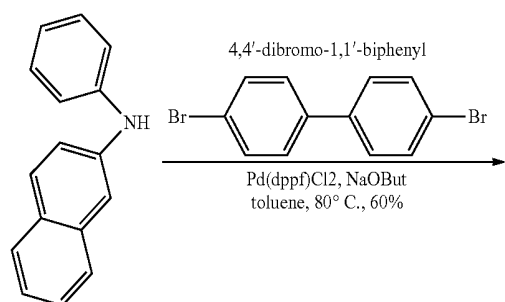
Compound 20
