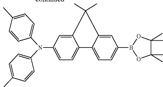
Compound 33
