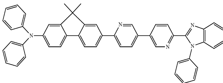
9,9-dimethyl-N,N-diphenyl-7-(6'-(1-phenyl-1H-benzo[d]imidazol-2-yl)-[3,3'-bipyridin]-6-yl)-9H-fluoren-2-amine,
